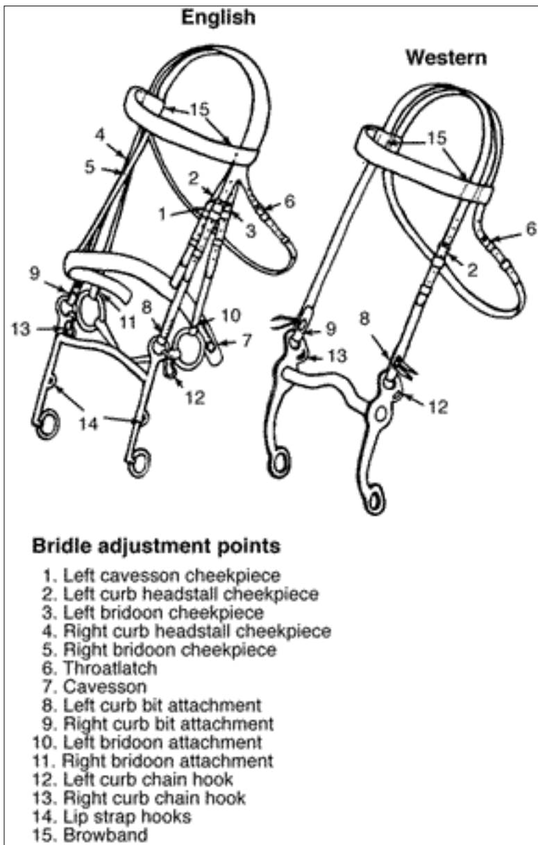
Figure 1. Bridle nomenclature and adjustment points.
